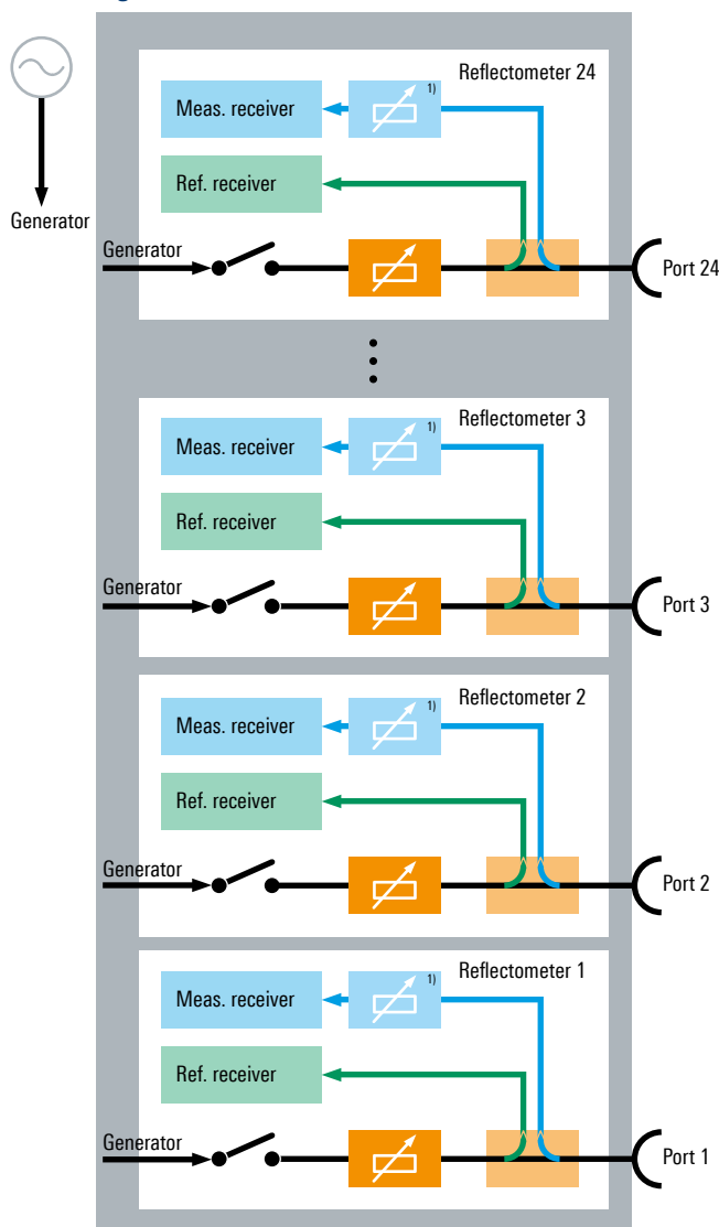
Block diagram of an R&S®ZNB
