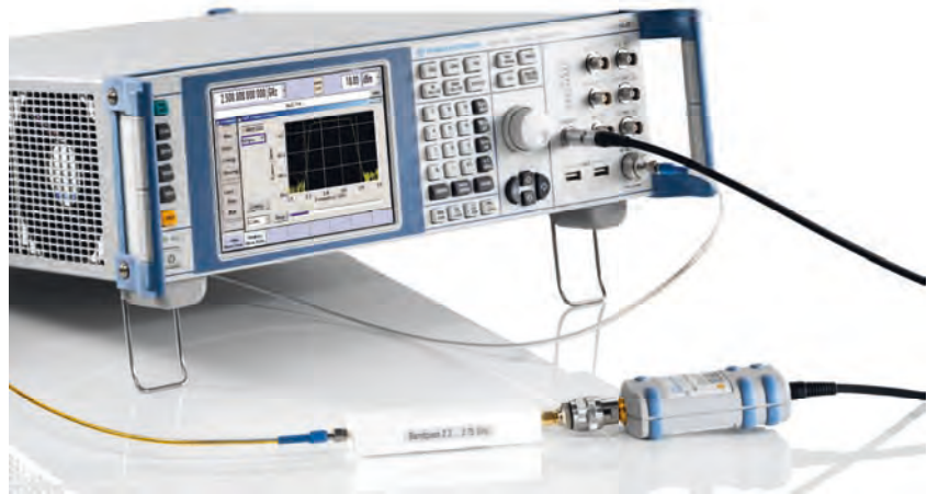
Scalar network analysis on an external bandpass filter (with R&S®SMF-K28 power analysis option plus R&S®NRP-Zx power sensor)
