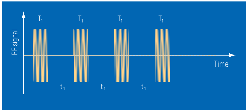
Single pulses
