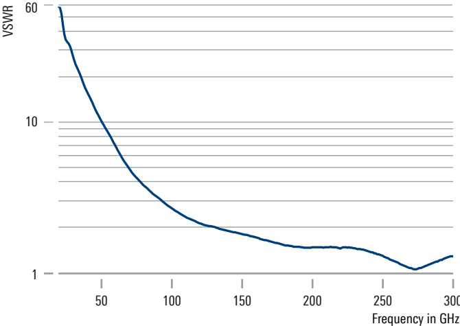
Typical VSWR
