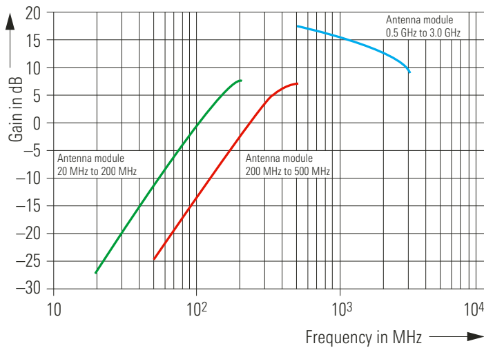
Typical practical gain in active mode
