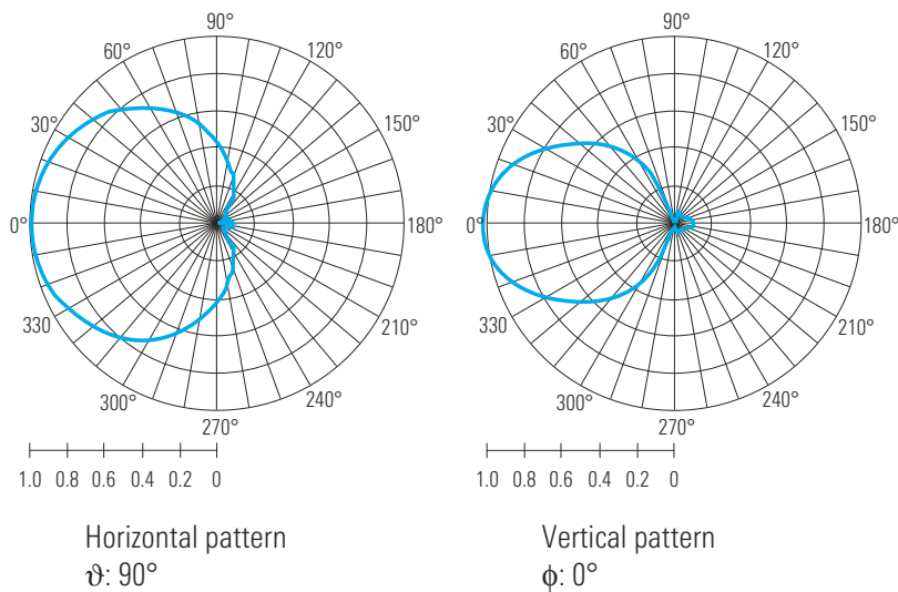
Typical directional radiation pattern in the frequency range 0.5 GHz to 3 GHz
