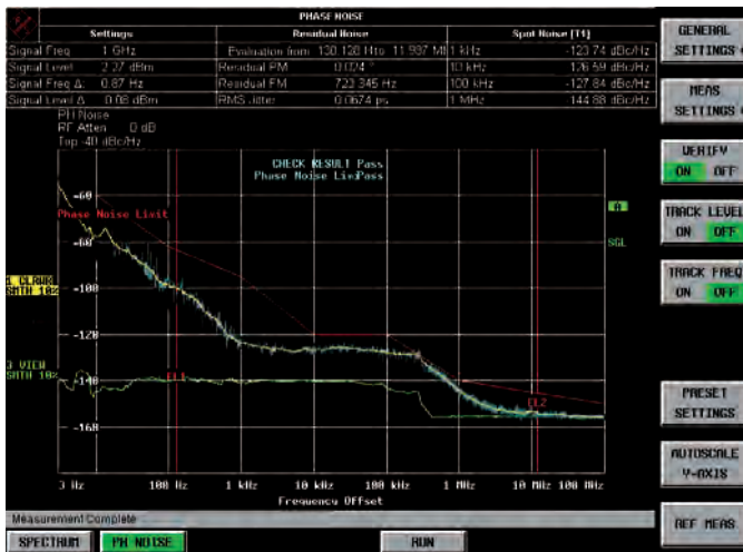
Phase noise measurement with the R&S®FS-K40 application firmware.
