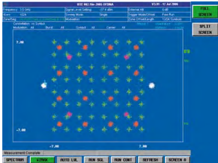
Constellation diagram with low signal-to-noise ratio.
