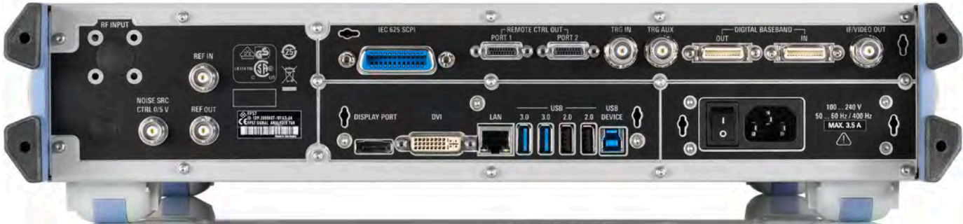
All R&S®FPS ports are located on the rear panel, making it ideal for integration into rack systems.
