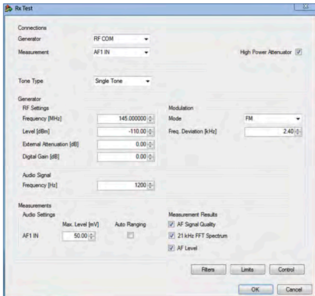
Configuration of R&S®CMArun test items.
