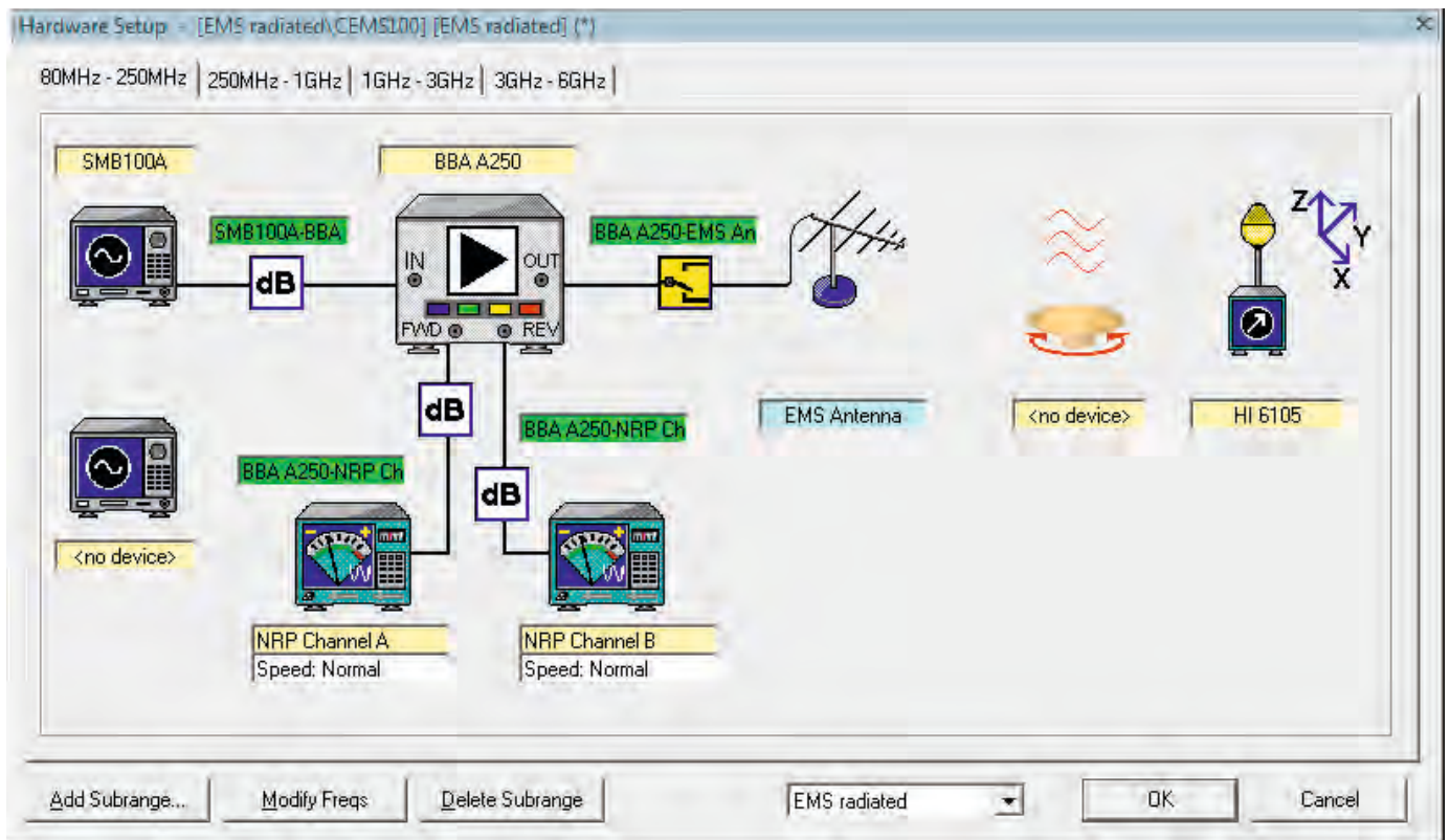
Configuration of disturbance signal generation with an R&S®CEMS100 for EMS testing.
