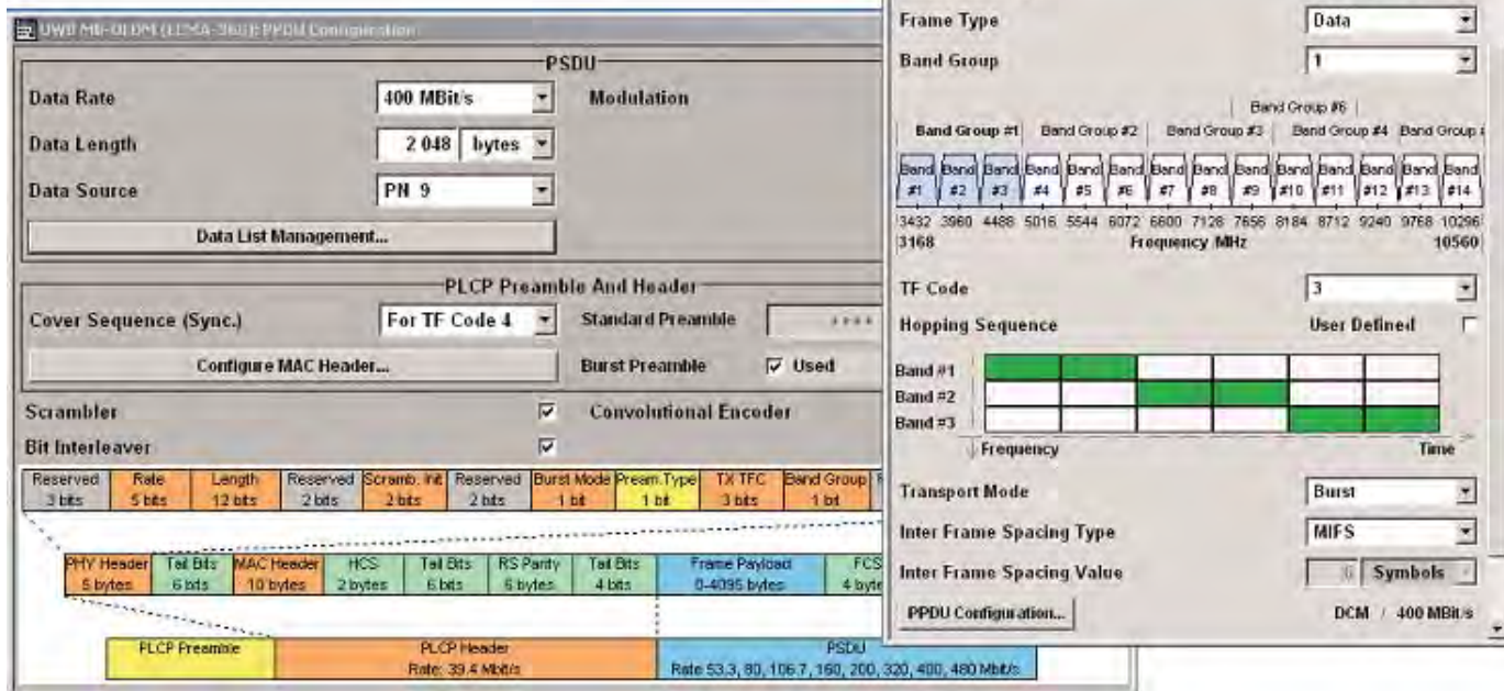
R&S®AFQ-K264 option for UWB (ECMA-368)
